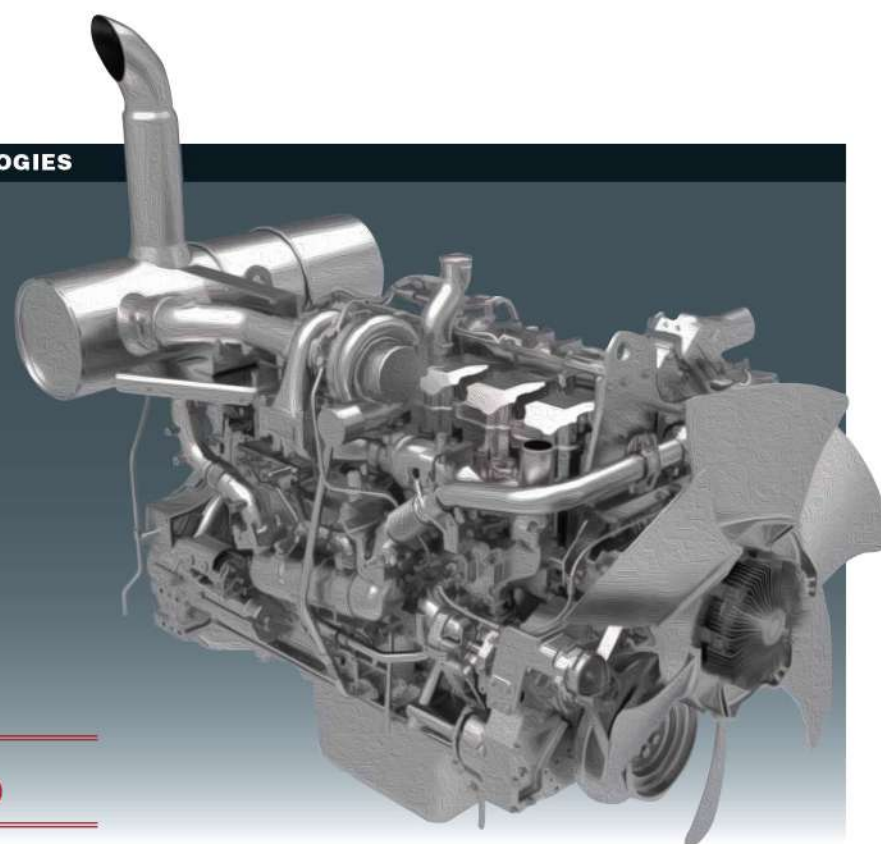
Komatsu SAA6D125E-5 engine EU Stage 3A emission equivalent. (CG image)
